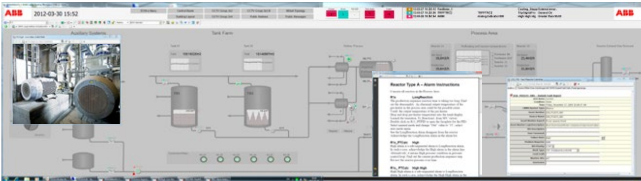
Live Video and CMMS Maximo seamless integrated in the process display
